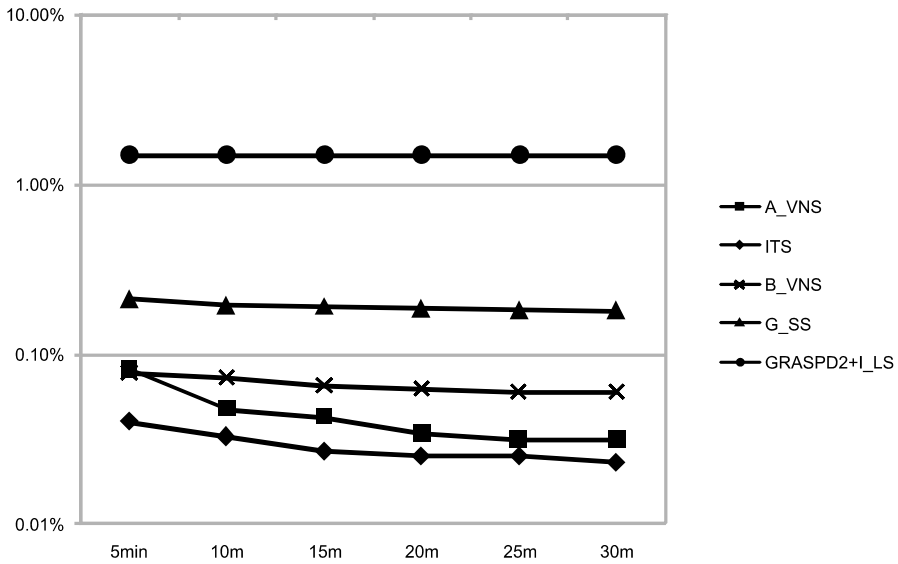
Fig. 1 Search profile for a 30-minute run of the largest instances
